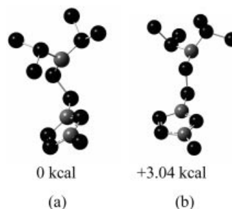
Figure 2. Calculated energies of two structures at the B3LYP/6-311+G** level of theory [dihedral angle N5–N7–C8–N9 in (a) single crystal 69.6°; in (b) 180°].
