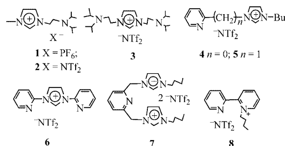
Scheme 1. Structures of basic ionic liquids.
