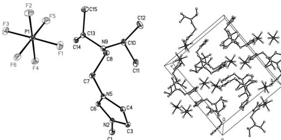
Figure 1. Thermal ellipsoid plot (30%) (left) and packing diagram (right) of 1 .
