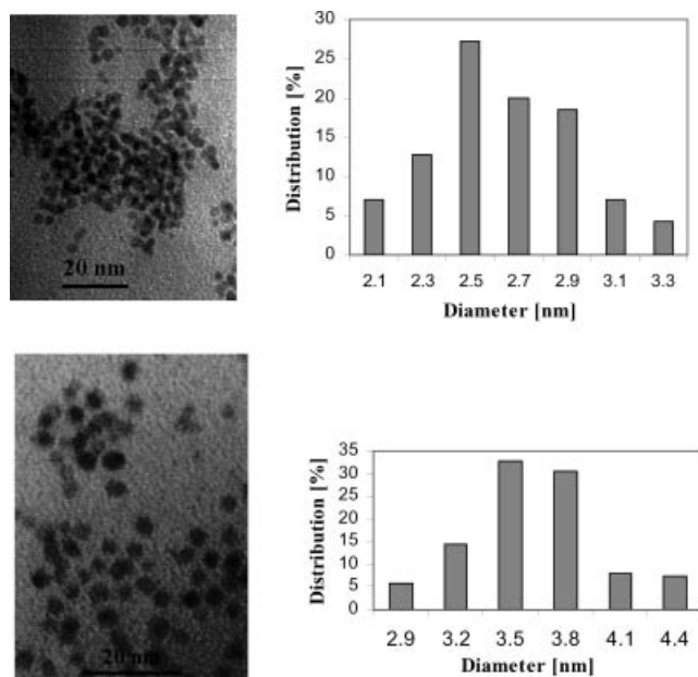
Figure 3. TEM and size distribution of Pd nanoparticles formed in THF (upper) and acetone (lower).
